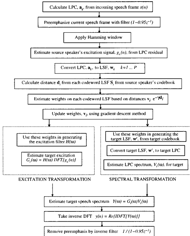
Figure 1: Flow-diagram of STASC voice conversion algorithm.
