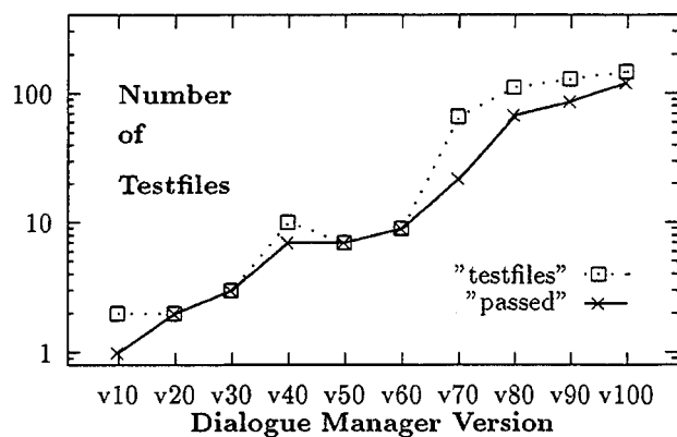
Figure 4: Dialogue Manager Progress
