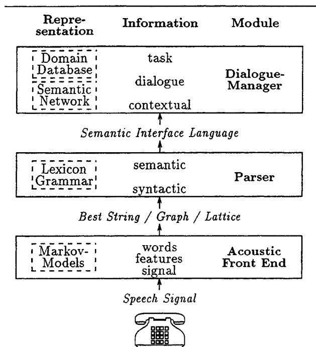
Figure 1: Processing Stages in SUNDIAL
