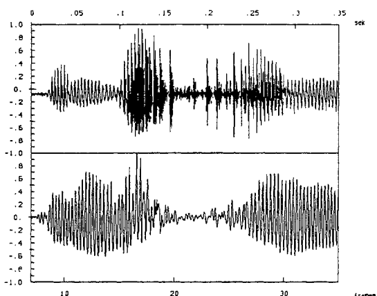
Figure 6: Speech signal and ANN-VSS of a speaker in data set B (no reference VSS available).
