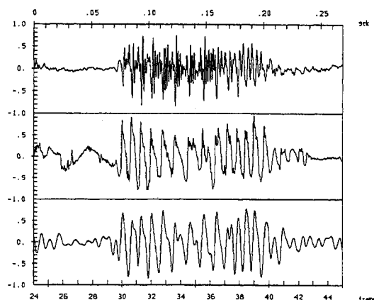
Figure 3: Speech signal, voice source signal and ANN-VSS of the training set L1.
