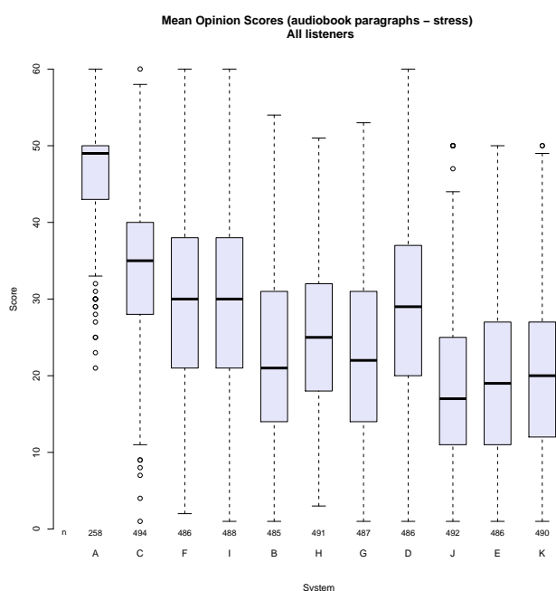
Figure 7: Stress assignment results (D - GlottHMM).
