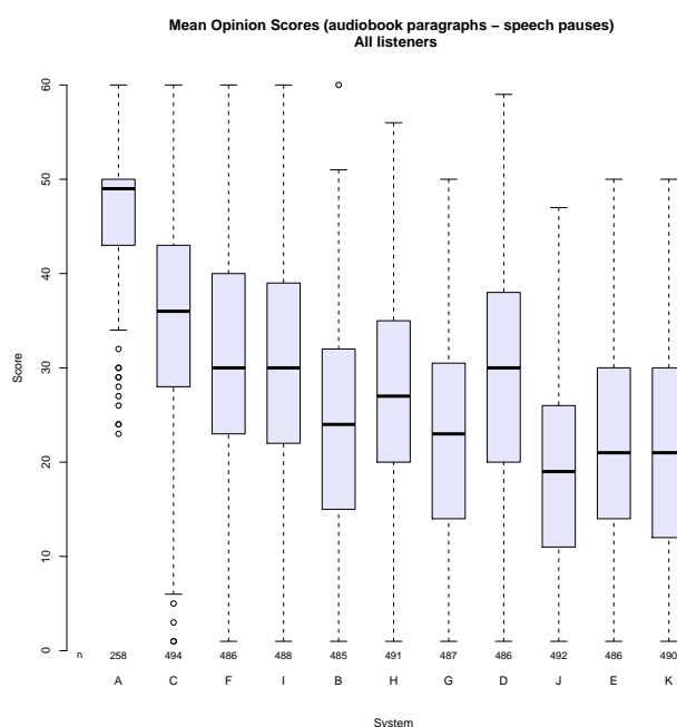
Figure 8: Pause results (D - GlottHMM).
